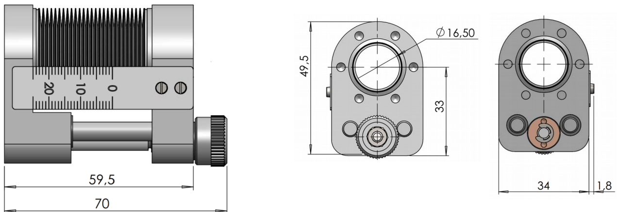
Side view, top view and bottom view with important dimensions
