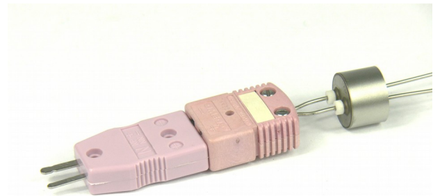
Connector with adaptor to use with a female miniature connector
