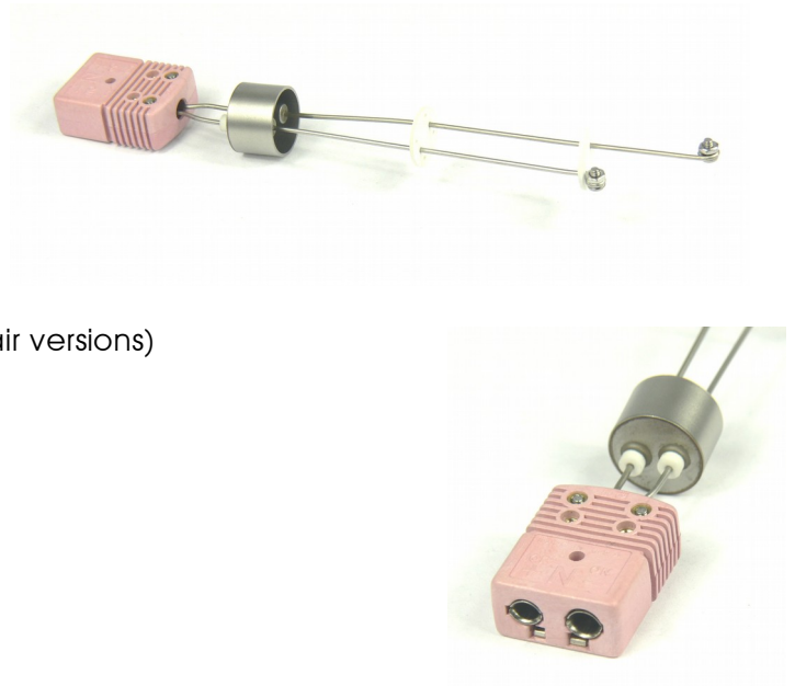
Fitted connector on a weldable feedthrough, visible is the option to insert standard or miniature male connectors
